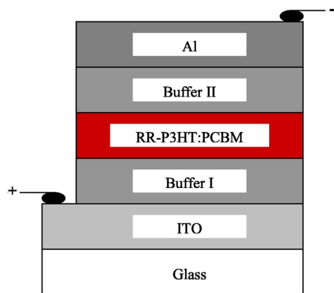
FIG. 1. (Color online) (a) Schematic of the device structure of polymer solar cell fabricated in this study and (b) the molecular structures of active materials in polymer solar cell—RR-P3HT and PCBM.
