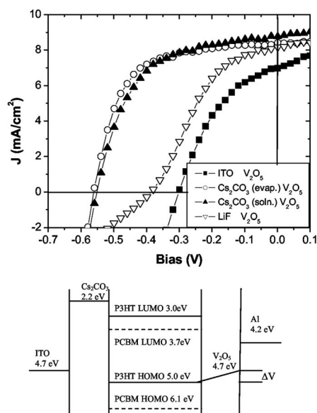
FIG. 3. (a) Current-voltage characteristics of inverted polymer solar cells. The interfacial layers and blend/Al interfaces are (i) none, \text{V}_2\text{O}_5 (solid square); (ii) \text{Cs}_2\text{CO}_3 (evaporated), \text{V}_2\text{O}_5 (open circle); (iii) \text{Cs}_2\text{CO}_3 (solution process), \text{V}_2\text{O}_5 (solid triangle); and (iv) LiF, \text{V}_2\text{O}_5 (open inverted triangle). (b) Energy level diagrams for various materials in the inverted solar cells.
