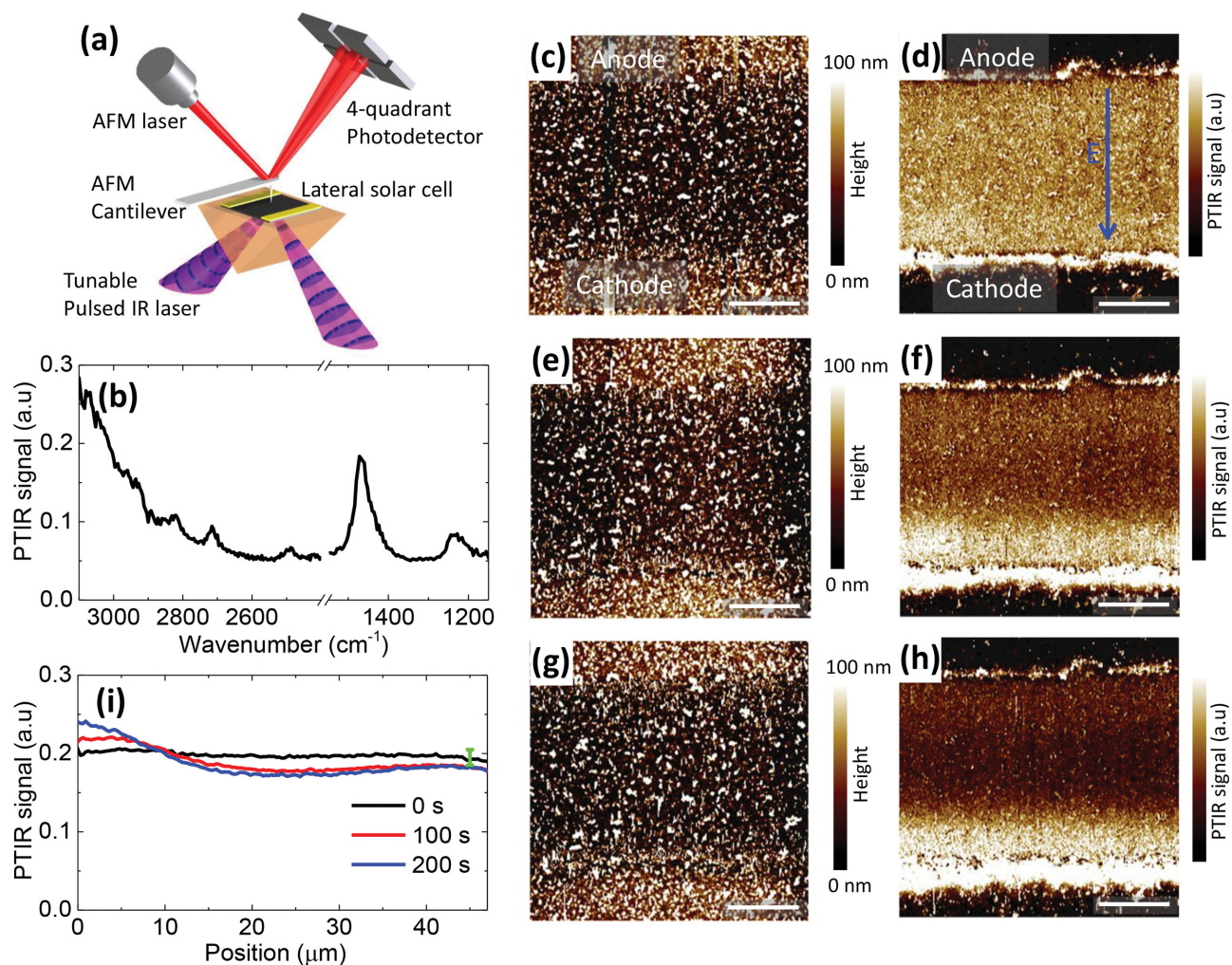
Figure 2. a) Schematic illustration of the PTIR measurement. b) A representative absorption spectrum obtained at the center of the device. c,e,g) Topography maps ( 80 \mu\text{m} \times 80 \mu\text{m} ) of the \text{MAPbI}_3 film of the same sample area before (c), after 100 s (e) and after 200 s (g) electrical poling, respectively. The poling field was 1.6 \text{ V } \mu\text{m}^{-1} . d,f,h) Corresponding PTIR images for the \text{CH}_3 asymmetric deformation absorption of the methylammonium ion ( 1468 \text{ cm}^{-1} ) obtained before (d), after 100 s (f) and after 200 s (h) electrical poling, respectively. i) Line-averaged profile (perovskite region only) of 256 vertical lines in the PTIR images before and after electrical poling, showing the redistribution of the \text{MA}^+ ions. The error bar represents the uncertainty of the background level when comparing data from different scans. All scale bars are 20 \mu\text{m} .
