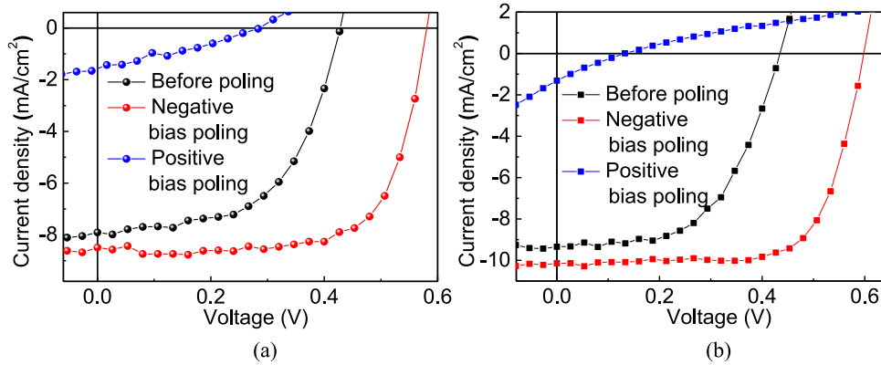
Fig. 2. (a) Photocurrent of the P3HT:PC 60 BM device before and after negative bias poling with TPACA as cathode interfacial layer. (b) Photocurrent of the P3HT:PC 60 BM device before and after poling with TPACA blended in the active layer.
