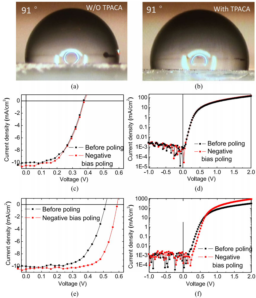
Fig. 3. Contact angle measurement of the PHT:PC 60 BM film (a) without and (b) with TPACA blended in the active layer. (c) Photocurrent and (d) dark current of the device before and after negative bias poling after methanol washing with TPACA as interfacial layer. (e) Photocurrent and (f) dark current of the device before and after negative bias poling after methanol washing with TPACA blended in the P3HT:PC 60 BM active layer.
