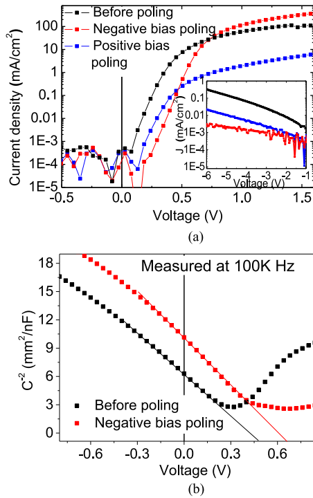
Fig. 4. (a) Dark current of the device with TPACA blended in the active layer. The inset is the dark current of the device under negative bias. (b) Built-in potential of the P3HT:PC 60 BM device measured by fitting the 1/C^2 versus voltage curve.
