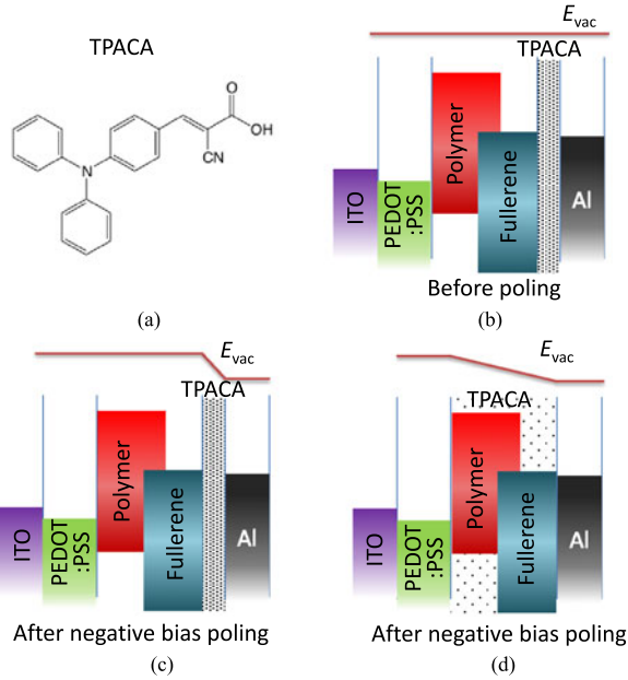
Fig. 1. (a) Molecular structure of TPACA. Energy diagram of the device (b) before poling and (c) after negative bias poling with TPACA as the cathode interfacial layer. (d) Energy diagram of the device after negative bias poling with TPACA blend in the active layer.
