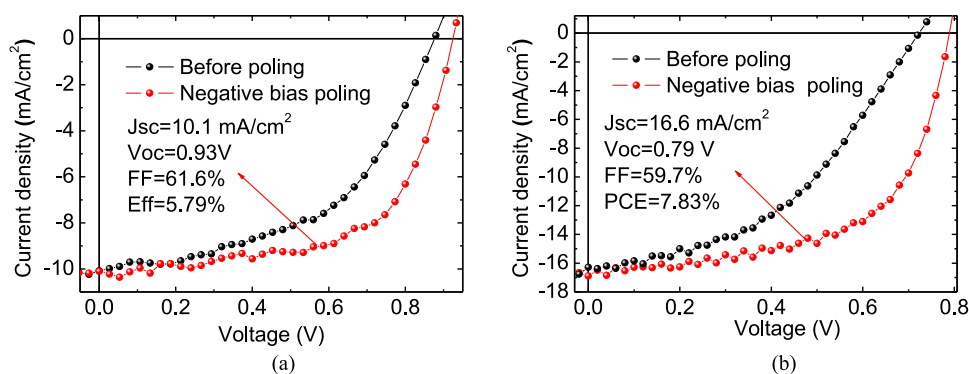
Fig. 6. TPACA polar molecule application in (a) PCDTBT:PC 70 BM system and (b) PBDTTT-CT:PC 70 BM system with TPACA blended in the active layer.
