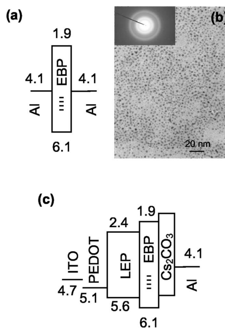
FIG. 3. (a) Schematic energy diagram of polymer bistable device, (b) TEM image of dodecanethiol capped gold nanoparticles with size distribution from 1.6 to 4.4 nm, and, (c) schematic energy diagram of polymer bistable LED with the HOMO and LUMO levels of materials used and trap levels of dodecanethiol capped gold nanoparticles (short lines), in electron volts and with respect to vacuum level.
