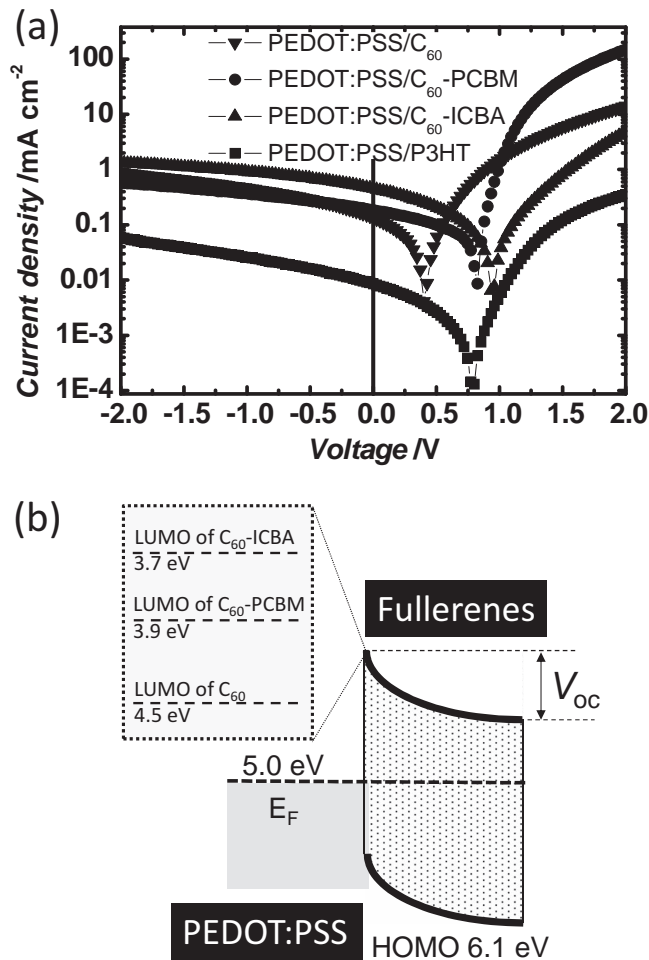
Figure 1. a) J - V curves of C_{60} -, C_{60} -PCBM- and C_{60} -ICBA-based Schottky junction devices. b) Schematic energy diagram showing the variation of V_{oc} of C_{60} -, C_{60} -PCBM- and C_{60} -ICBA-based Schottky junction devices. For better clarity, the energy levels were not drawn in scale.
