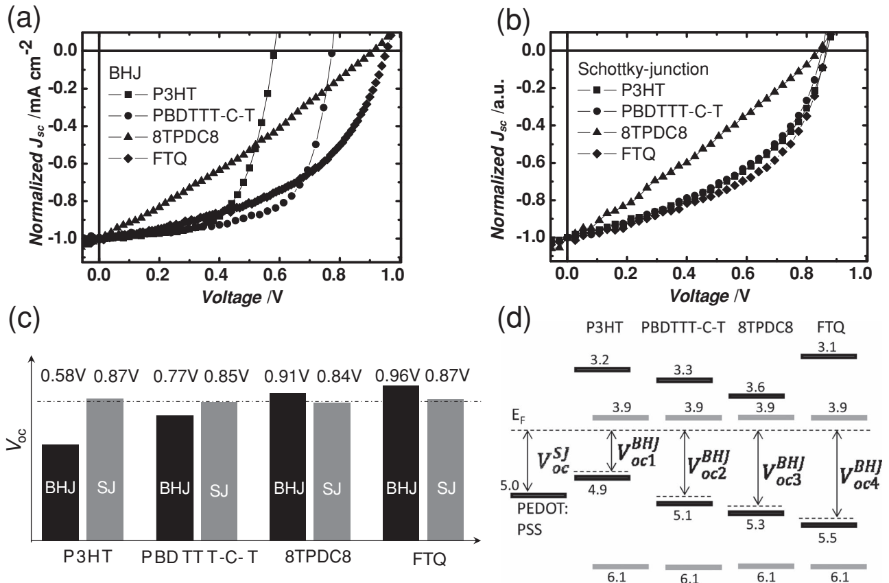
Figure 3. a,b) Normalized photocurrent curves of the BHJ devices (a) for different donors and Schottky junction (SJ) devices (b) for different donors, with donor polymers P3HT (50 wt% for BHJ, 5 wt% for SJ), PBDTTT-C-T (50 wt% for BHJ, 5 wt% for SJ), 8TPDC8 (50 wt% for BHJ, 5 wt% for SJ), and FTQ (40 wt% for BHJ, 5 wt% for SJ). c) The measured V_{oc} of SJ and BHJ devices. d) Comparison of the energy diagram of V_{oc} determined by SJ and BHJ; the black bars represent the donor materials, the grey bars represent C 70 -PCBM.
