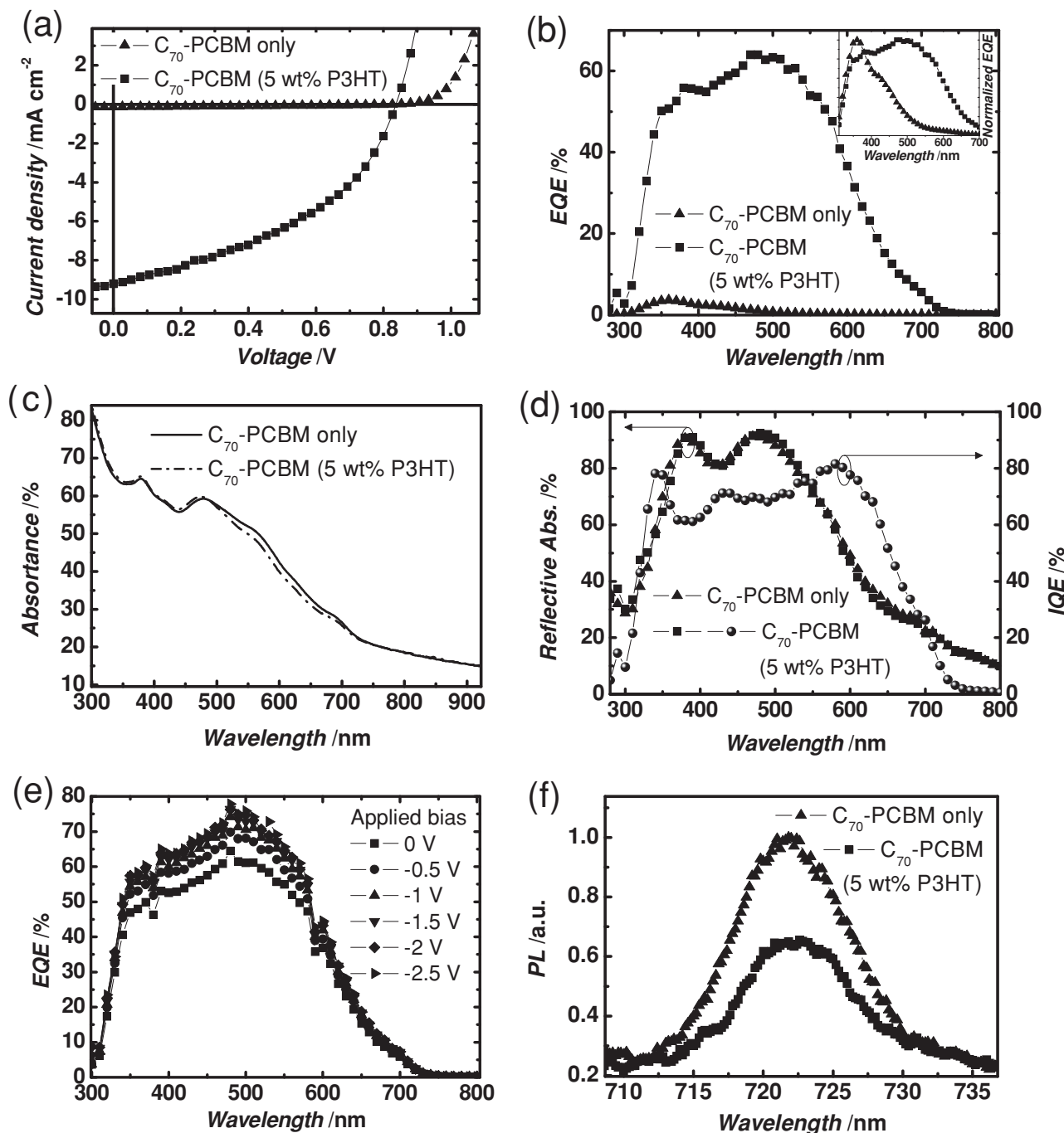
Figure 2. a,b) The photocurrent curves (a) and EQE curves (b) of Schottky junction devices based on pure C 70 -PCBM and C 70 -PCBM:P3HT (95 wt%:5 wt%). c) The transmission absorption spectra of C 70 -PCBM-only film and the blend film C 70 -PCBM:P3HT (95 wt%:5 wt%). d) The IQE (right) and reflective absorption spectra (left) of C 70 -PCBM-only- and C 70 -PCBM:P3HT (95 wt%:5 wt%)-based devices. e) The EQE curves of the Schottky junction device based on C 70 -PCBM:P3HT (95 wt%:5 wt%) under different reverse biases. f) The PL spectra of the C 70 -PCBM-only film and the C 70 -PCBM:P3HT (95 wt%:5 wt%) blend film.
