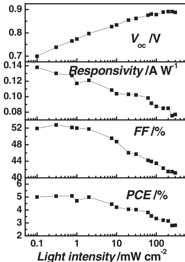
Figure 4. The variation of the photovoltaic parameters with light intensity for the Schottky junction device with C_{70} -PCBM:P3HT (95:5 wt%) as the active layer.
